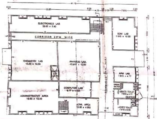
COMP. GROUND FLOOR PLAN (SCALE = 1:100)
