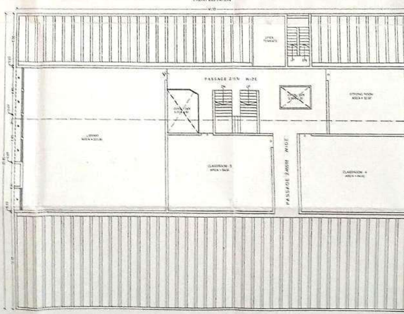
SECOND FLOOR PLAN SCALE 1:100
