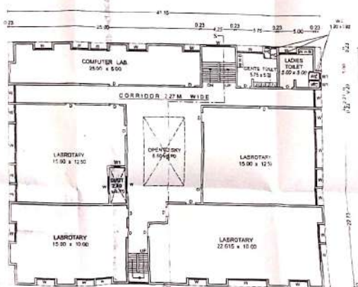
COMP. FIRST FLOOR PLAN
